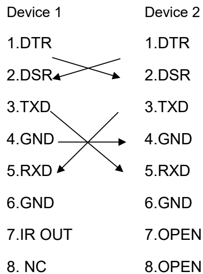
Figure1-7 VISCA Networking Diagram
