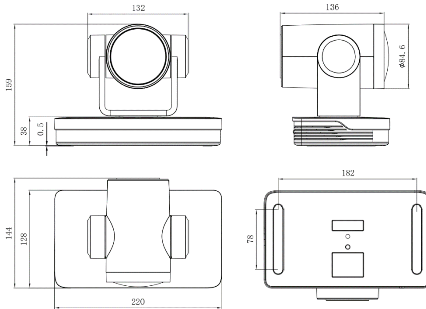
Figure1-4 Product Dimension
